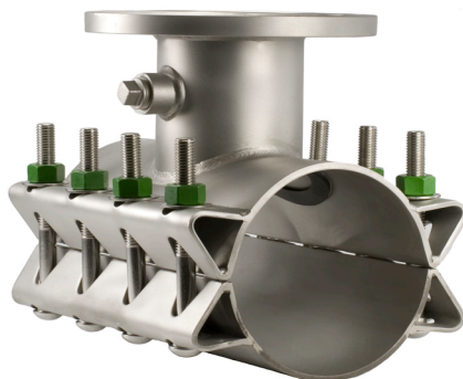
JCM 6452 Tapping Sleeve Image reflects 6" x 4"
